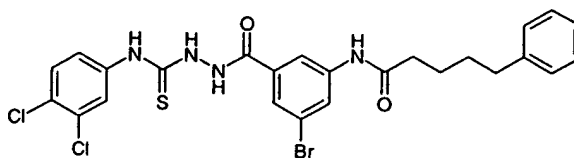
Compound # 53
